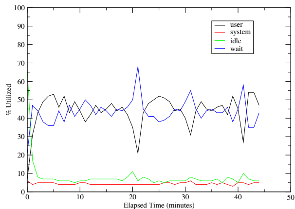
Figure 8: DBT-2 Processor Utilization
