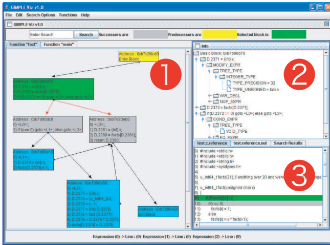
Figure 4: Gimple Viz displaying a file. 1 marks the CFG area, 2 marks the tree view, and 3 marks the source/search area.
